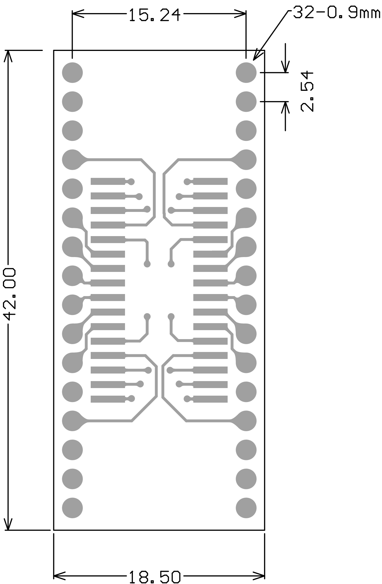
i2PA0126AA Dimensions t=1.6mm
