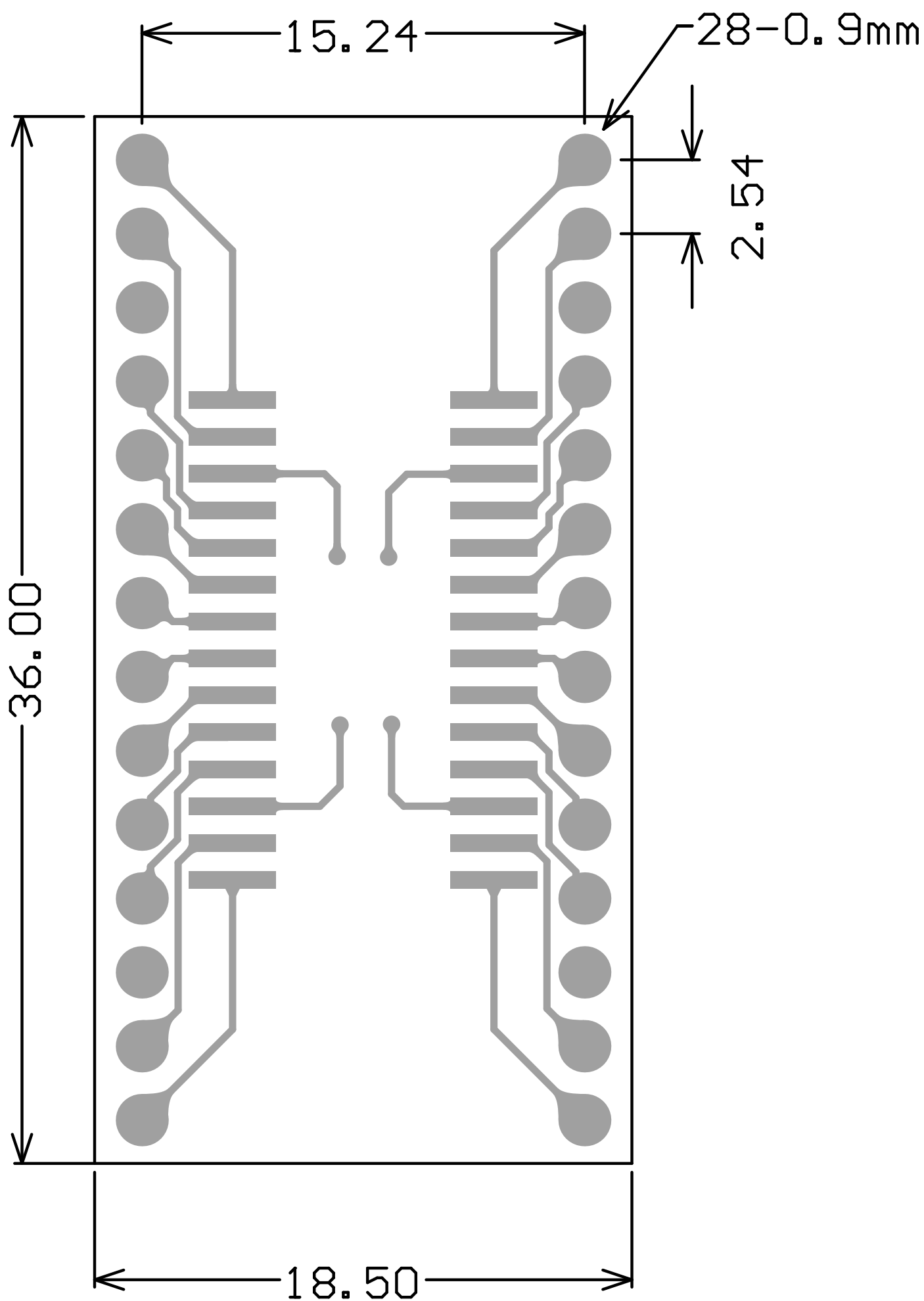
i2PA0125AA Dimensions t=1.6mm
